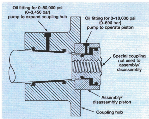
Fig. 2. Fluid supplied through drilled porting.
